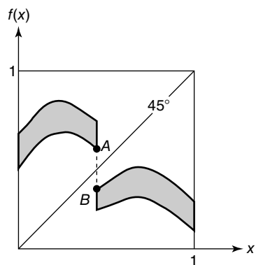
(a) Correspondence that is not convex
