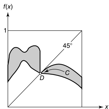
(b) Correspondence that is not upper semicontinuous
